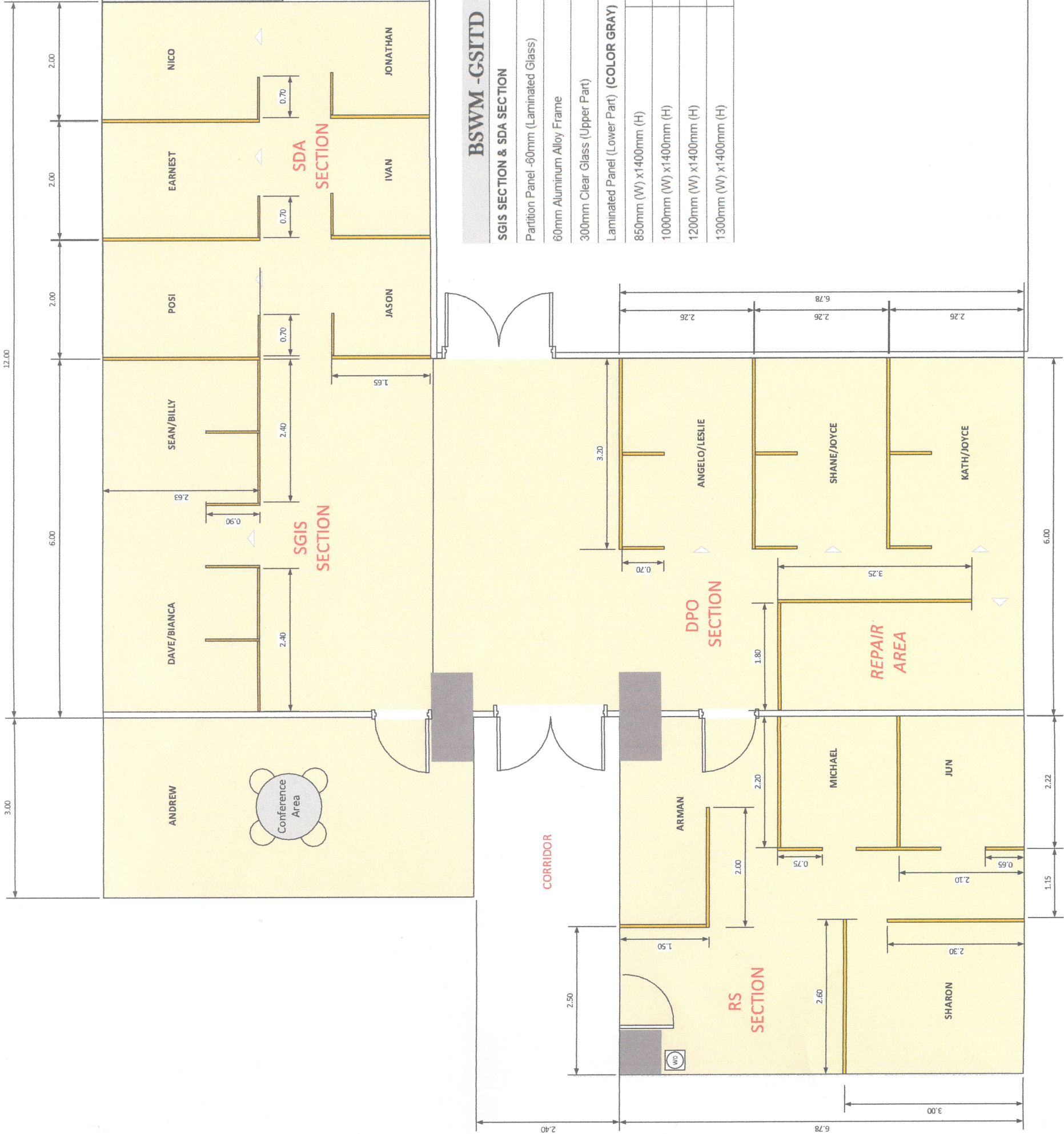
LAYOUT OF DIVIDER (SECOND FLOOR) SCALE 1:50 M
