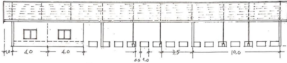
3 LEFT SIDE VIEW SCALE: 1:125 M.
